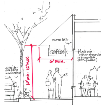
Figure 4-15: Overhangs should extend over roughly half of sidewalks.
