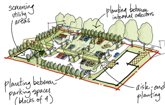
Figure 4-4: Support pedestrian movement, safety and comfort in parking areas.
