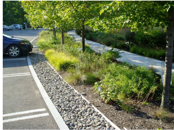
Image 16: Pervious, landscaped surfaces and light reflective surfaces minimize heat absorption.
