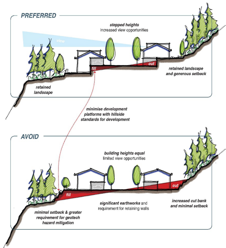
Figure 2-1: Developments should accommodate grade transitions within building design.
